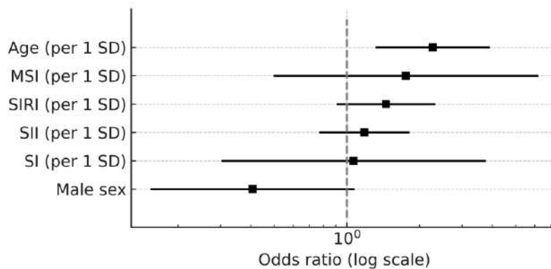
Figure 2. Adjusted odds ratios in the multivariate logistic model
