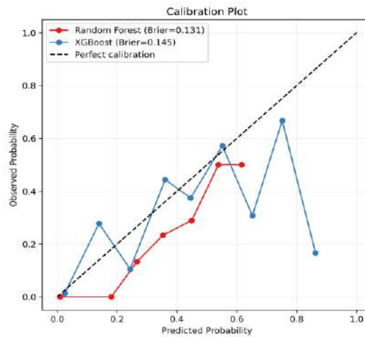
Figure 2. Calibration curves for the Random Forest (Brier = 0.131) and XGBoost (Brier = 0.145) models on the hold-out test set.
